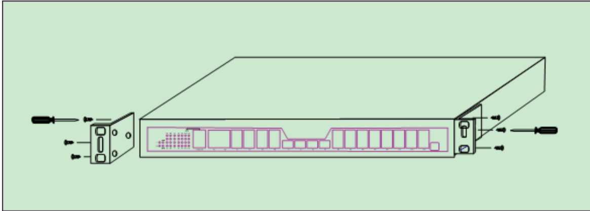
Figure 3-1 Fixing the machine box of TR- GP3600-08 GPON to the cabinet
