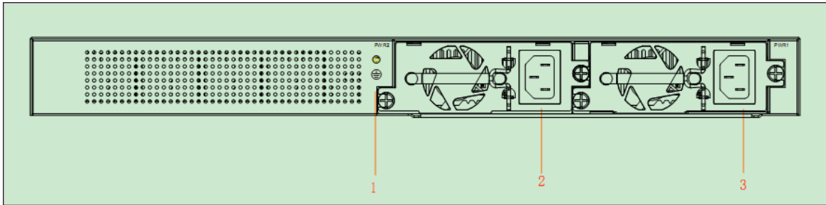
Figure 1-2 Back faceplate of GP3600-08 GPON-
